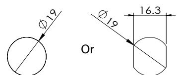
Hole drawing
